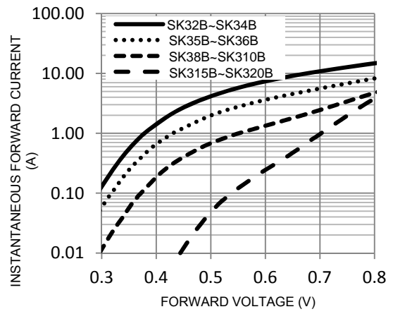
FIG. 2-Typical Forward Characteristics
