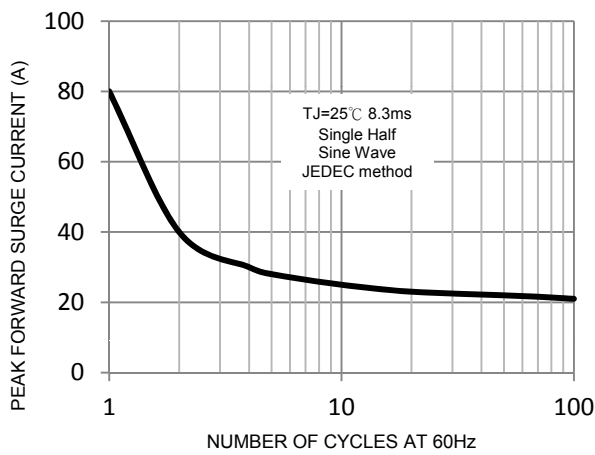
FIG. 3-Maximum Non-Repetitive Forward Surger Current
